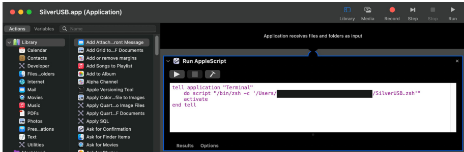
Figure 2: Automator to execute a backup script.
